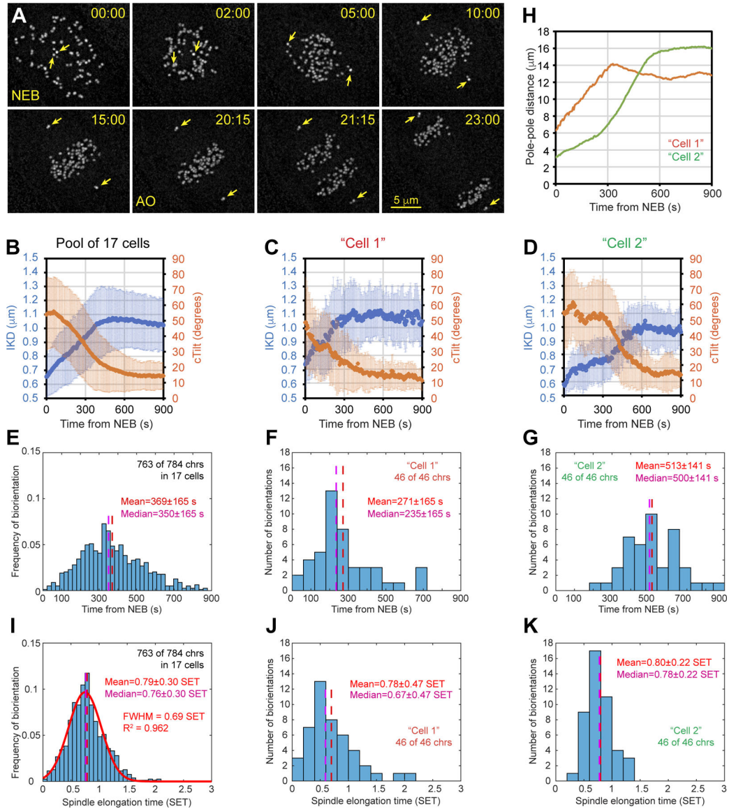
Figure 1. Amptelic attachments form at a specific stage of spindle elongation.
