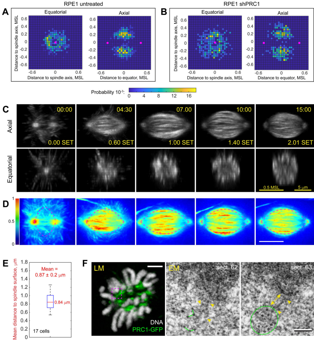
Figure 4. Amptelic attachments form within a spindle domain enriched in microtubule bundles. (A,B) Spatial distribution of biorientation events in the untreated (A) and PRC1-depleted (B) cells. 2D histograms in the Equatorial and Axial planes are shown. Distances are normalized to the Maximal Spindle Length in each cell. Magenta dots denote positions of spindle poles at the time with maximum probability of biorientation. (C) Selected timepoints from a timelapse recording of mitosis in RPE1 cells expressing PRC1-GFP. Axial and equatorial maximum-intensity projections of 3D volumes are shown. The volumes are aligned at each timepoint to stabilize the spindle position and orientation. Timestamps are in min:sec after NEB and in fraction of Spindle Elongation Time (SET). Scale bars are 5 \mu m and 0.5 of the Maximal Spindle Length (MSL) reached in this cell. (D) Average of 3-D time-lapse recordings aligned as in (A) and spatially normalized by the Maximal Spindle Length in each cell. Color map encodes intensity of PRC1-GFP in the averaged volume. Dashed lines approximate the edge of PRC1-enriched domain by an empirically constructed catenary
