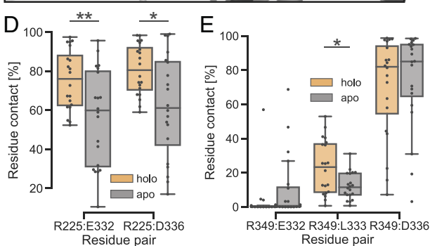
Fig. 3. ATP allosterically influences parvin-binding salt bridges. (A) Residue-based, pairwise forces compared between ILK holo and apo with different force thresholds (purple lines). Approximate positions of the ATP-binding pocket (orange arrow) and salt-bridge-forming arginines R225 and R349 (purple arrows) are shown. (B and C) Proposed force transduction pathways from ATP to salt-bridge-forming arginines R225 and R349, respectively, and into parvin and as calculated by FDA (for force values, see SI Appendix , Fig. S4). (D) Trajectory-averaged residue contact probability (threshold 0.35 nm) between ILK R225 and parvin depending on the presence of ATP ( n = 20 independent trajectories). **P = 0.0096 ; *P = 0.013 (Mann-Whitney). (E) Residue contact probability between ILK R349 and parvin as in D ( n = 20 independent trajectories). *P = 0.017 (Mann-Whitney).
