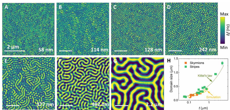
Fig. 2. MFM measurements at room temperature. (A to G) MFM images of an FCGT nanoflake on a SiO 2 /Si substrate with different thicknesses (scale bar, 2 \mu\text{m} ). The thickness was measured by atomic force microscopy. (H) Domain size as a function of the FCGT thickness. The skyrmion size strongly depends on flake thickness. The dotted line is a fit to Kittel's law. The micromagnetic simulation results also follow Kittel's law (yellow circles).
