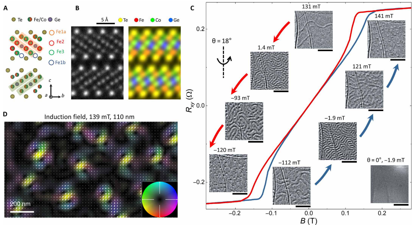
Fig. 1. Skymion creation as a function of the out-of-plane magnetic field at room temperature. (A) Structural model of FCGT viewed along the a axis. Fe1a site, Fe2 site, Fe3 site, and Fe1b site are marked by orange, red, green, and blue circles, respectively. (B) Experimental atomic resolution HAADF-STEM image (left) and the corresponding STEM–energy-dispersive x-ray spectroscopy (EDS) map (right). The STEM-EDS map is shown as a composite overlay of Fe, Co, Ge, and Te with red, green, blue, and yellow color maps, respectively. (C) Hysteresis curve of a 110-nm-thick FCGT flake and the corresponding Lorentz TEM images at various applied fields. The red (blue) curve indicates the direction for decreasing (increasing) magnetic fields. The contrast change between 0° and 18° tilt reveals the Néel character. Scale bars, 500 nm. (D) Magnetic induction field map of isolated skyrmions in a 110-nm-thick flakes obtained using 4D-LSTEM along with an EMPAD, with applied fields of 139 mT. The color and arrows indicate induction field components perpendicular to the beam propagation direction of Néel skyrmions at an 18° tilt.
