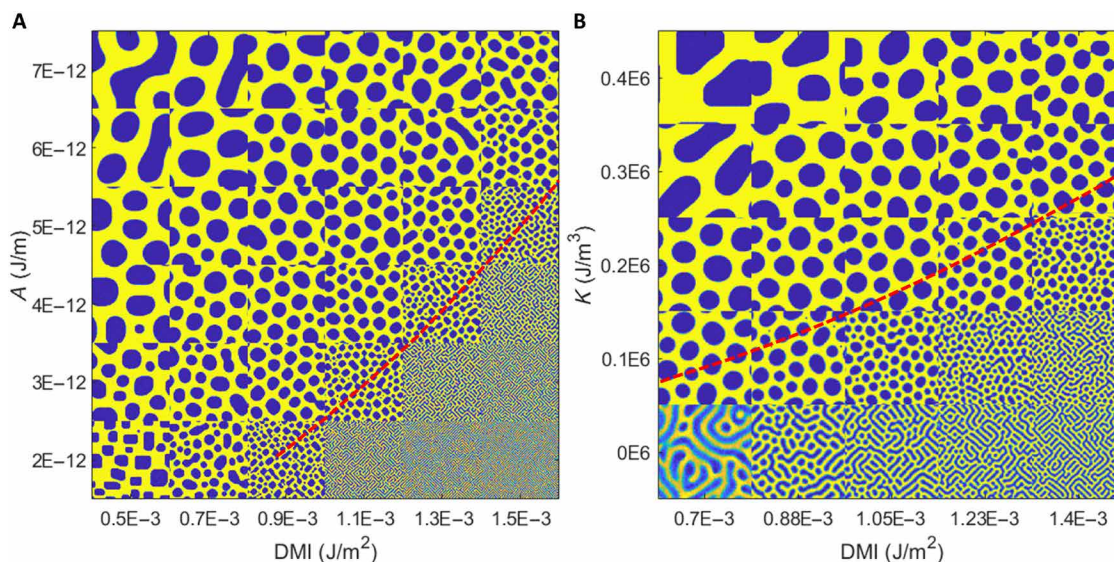
Fig. 4. Micromagnetic simulations. (A) Skymrion phase diagram as a function of DMI constant D and exchange stiffness constant A in 200-nm FCGT. (B) Skymrion phase diagram as a function of DMI constant D and effective PMA energy K . We have used a 4-nm maximum distance between unit cells, which is lower than the value of the exchange length l_{ex} = \sqrt{\frac{2A}{\mu_0 M_s^2}} \sim 9.8 nm. The image size is 1 \mu\text{m} by 1 \mu\text{m} . The red dashed line follows the solution of \sigma_w = 0 .
