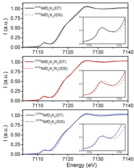
Fig. 3 Comparison of the normalized Fe K-edge XAS spectra of \Delta^{HADZ} NifD 2 K 2 (top), \Delta^{HADZ} NifD 2 K 2 W 2 (middle), and C^{275A} NifD 2 K 2 (bottom) in the DT-reduced (solid) and IDS-oxidized (dashed) forms. Insets show an expanded view of the pre-edge region from 7109–7116 eV.
