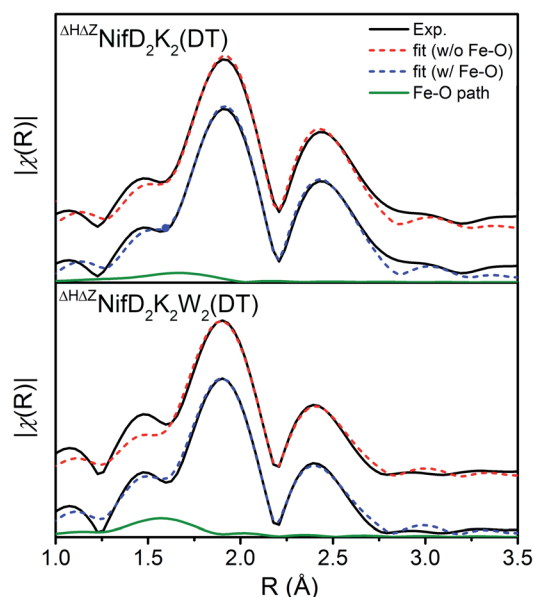
Fig. 5 Comparison of the Fe K-edge EXAFS of DT-reduced {}^{\Delta H\Delta Z}NiFD_2K_2 (top) and {}^{\Delta H\Delta Z}NiFD_2K_2W_2 (bottom) experimental spectra (black) and respective best fit models with (blue, dashed) and without (red, dashed) inclusion of an Fe–O/N scattering path contribution (green, solid). Corresponding fit parameters are provided in Table S1.† Spectra are k^2 -weighted, and FTs were performed for a k -range of 3–13 Å −1 . Fits were performed using k^3 -weighting over ranges of k = 3 –13 Å −1 and R = 1 –3 Å.
