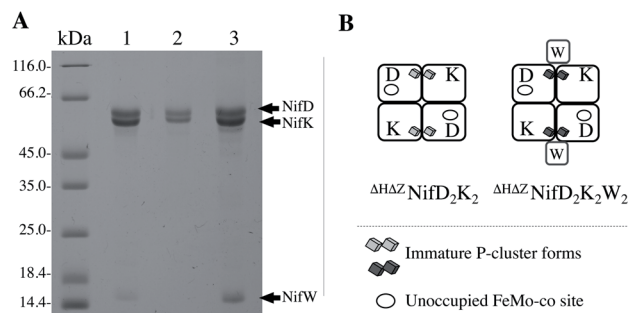
Fig. 2 NifD 2 K 2 species characterized in this work. (A) SDS-PAGE analysis of proteins isolated by one-step Strep-tag affinity purification (1), and \Delta^{HADZ} NifD 2 K 2 (2) and \Delta^{HADZ} NifD 2 K 2 W 2 (3) isolated by ion-exchange chromatography of the sample shown in (1). Molecular weight standards are shown on the left lane. The presence of a small amount of a \Delta^{HADZ} NifD 2 K 2 NafH x species (less than 8% of the total sample) in (3) was revealed by SDS-PAGE analysis of more concentrated samples as shown in Fig. S1.† (B) Schematic representation of samples shown in (A). Interaction of NifW at the interface of NifD 2 K 2 is only shown for convenience and has not been experimentally established. Corresponding X-band EPR spectra are provided in Fig. S2.†
