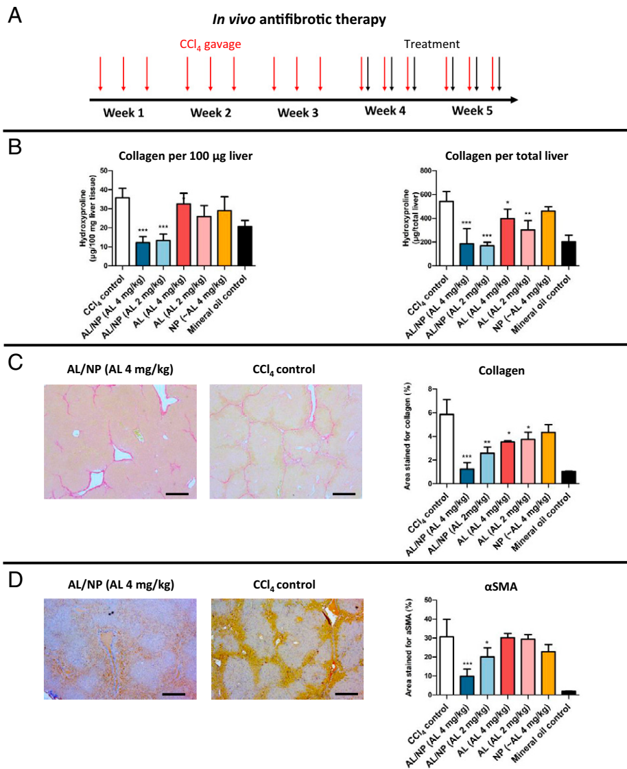
Fig. 4. In vivo antifibrotic effect of AL/NPs in CCl 4 fibrotic mice. (A) Treatment schedule for mice that were gavaged with CCl 4 three times a week for 5 wk. During the last 2 wk, mice received six intravenous injections of AL/NPs (2 or 4 mg/kg AL) or corresponding controls (unconjugated 2 or 4 mg/kg AL and NPs). 24 h after the final injection, mice were killed and livers were analyzed. (B) Collagen quantified by relative or total liver HYP content. (C) Morphometric assessment of collagen deposition in representative Sirius red–stained liver tissue sections (five randomly selected fields of each specimen omitting large vascular structures). (Scale bars, 200 \mu m.) (D) Morphometric assessment of \alpha -SMA+ myofibroblasts in representative liver sections (means \pm SD; * P < 0.05, ** P < 0.001, *** P < 0.0001 vs. CCl 4 fibrotic control mice; n = 5–7 in the treatment and CCl 4 fibrotic control groups, n = 4 in the mineral oil control group). (Scale bars, 200 \mu m.)
