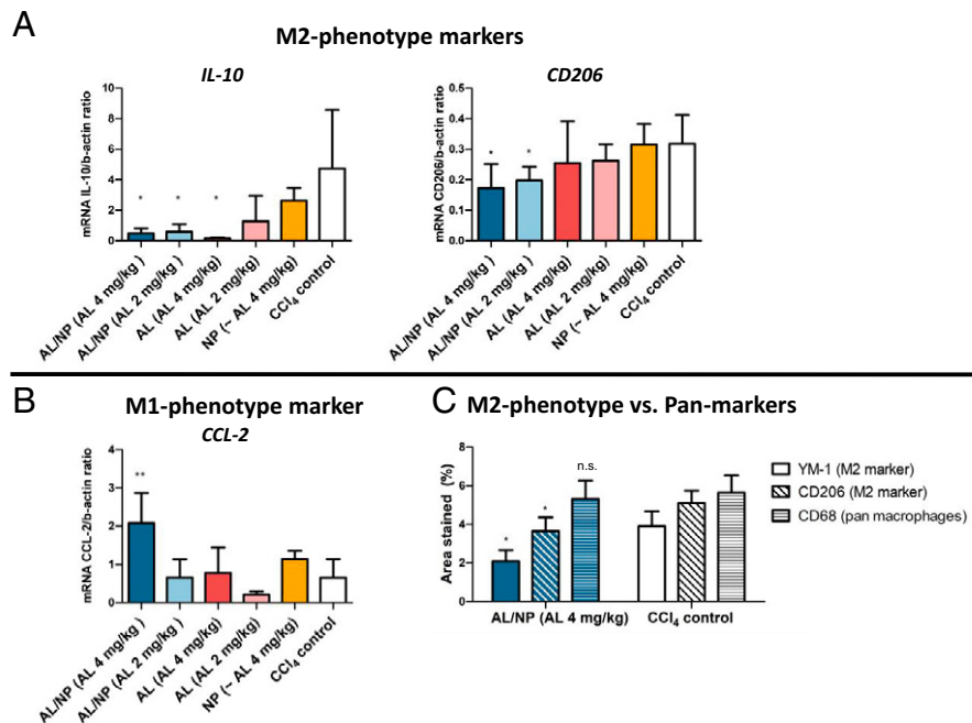
Fig. 6. Repolarization of M2 to M1 macrophage-phenotype markers by AL/NP treatment. (A and B) AL/NP treatment significantly reduced the M2-phenotype markers IL-10 and CD206 (A), while the M1-phenotype marker CCL2 was up-regulated (B) on the transcriptome as determined by qPCR ( *P < 0.05 , **P < 0.001 ). (C) In liver sections stained for the pan-macrophage marker CD68 or the M2 markers YM-1 and CD206, AL/NP treatment significantly reduced the M2-type markers YM-1 and CD206 on the protein level, while CD68 was not affected ( *P < 0.05 ; n.s., not significant).
