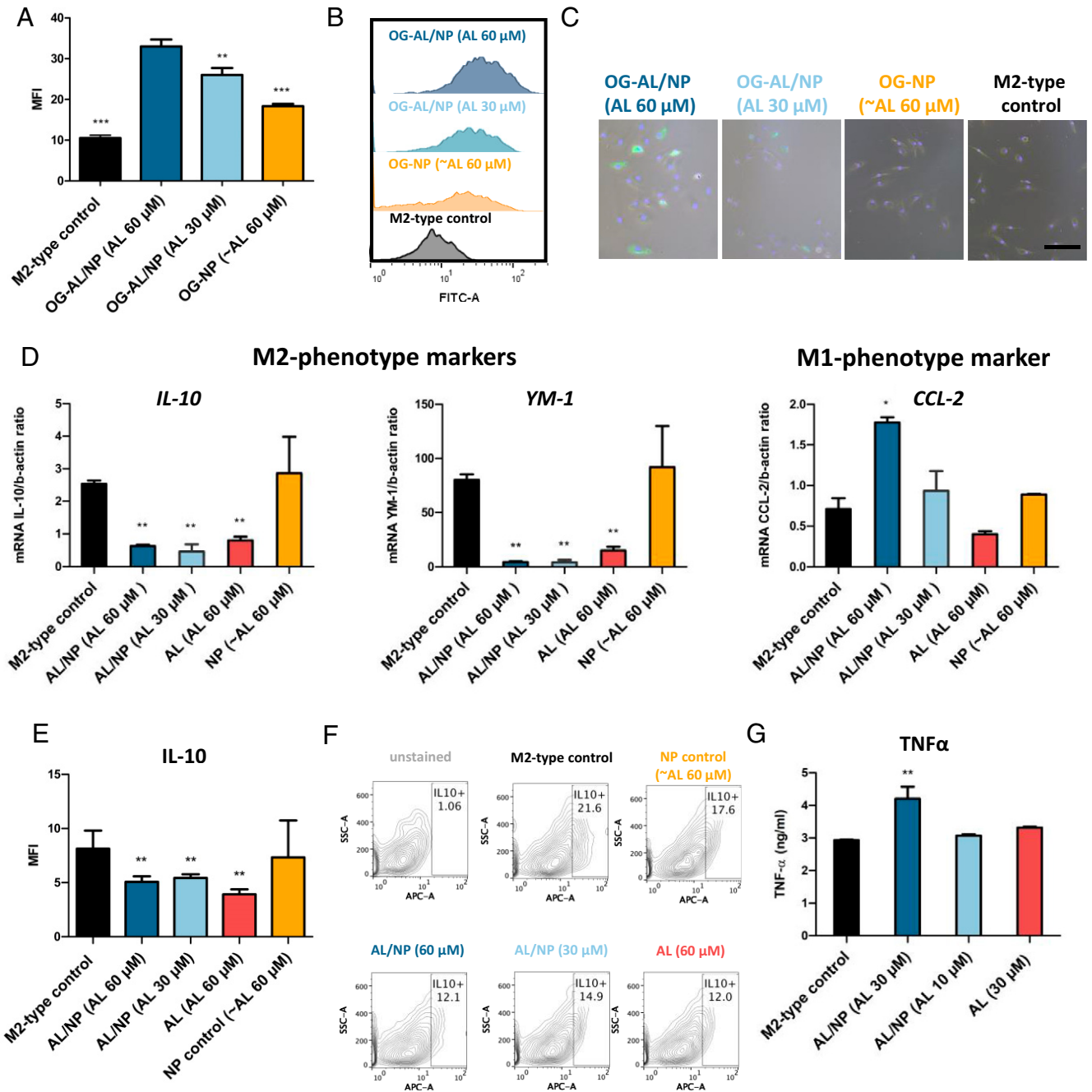
Fig. 2. In vitro performance of AL/NPs. (A) In vitro cellular uptake by mean fluorescence intensity (MFI) of OG-AL/NPs (30 and 60 \mu M AL) and control particle OG-NPs (at a representative concentration of \sim 60 \mu M AL) in M2-polarized primary macrophages (incubation time of 24 h, n = 3 , **P < 0.001 , ***P < 0.0001 , OG-AL/NPs vs. control). (B) Histograms of representative samples of A. (C) In vitro brightfield fluorescence microscopy of M2-polarized primary macrophages incubated with OG-AL/NPs (30 and 60 \mu M AL), OG-NPs, and untreated M2 macrophages as control (incubation time, 24 h). (Scale bar, 100 \mu m). (D) AL/NP treatment significantly reduces the transcript levels of the M2-phenotype markers IL-10 and YM-1 , while the M1-phenotype marker CCL2 was increased as determined by qPCR (incubation time, 48 h; n = 3 ; *P < 0.05 , **P < 0.001 vs. M2-type control). (E) AL/NP (30 and 60 \mu M AL) treatment significantly reduced IL-10 protein expression in M2-type primary macrophages as determined by flow cytometry (incubation time of 48 h, n = 3 , **P < 0.001 ). (F) Contour plots of representative samples of E. (G) Quantification of TNF \alpha protein levels in supernatants collected from M2-type macrophages treated with AL/NPs (30 and 10 \mu M AL) and controls (30 \mu M soluble AL or untreated) as determined by ELISA (incubation time of 48 h, n = 3 , **P < 0.001 ).
