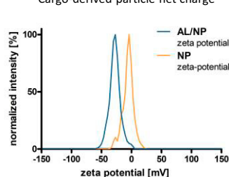
Fig. 1. Nanocarrier fabrication and characterization. (A) Background: Covalent AL conjugation can be achieved by squaric ester amides under aqueous conditions. (B) Macromolecular approach: Synthesis scheme of RAFT block copolymerization of the squaric ester amide methacrylamide monomer with a PEG-derived chain transfer agent. (C) Supramolecular design: Scheme of nanogel fabrication from self-assembled squaric ester amide-based precursor micelles through sequential functionalization, including pH-responsive cross-linking, fluorescent dye labeling, and drug loading. Subsequent pH-triggered degradation can be afforded through acid-promoted hydrolysis of the ketal cross-linkers. (D) AL load quantification of AL/NPs using photometric phosphate assay and 31 P NMR. (E) Ultrasensitive pH-triggered disassembly: DLS count rate of AL/NPs upon exposure to pH 7.8 compared to mildly acidic values of pH 6.8, 6.4, 6.0, and 5.2 over time. DLS size distribution of AL/NPs before (0 min, dotted line), as well as upon exposure to the different pH values (300 min, solid line). (F) Zeta potential of bisphosphonate-loaded AL/NPs compared to control NPs. (G) Stability in human plasma: FCS study of AL/NPs after 0 and 24 h of incubation in human blood plasma. R H , hydrodynamic radii.
