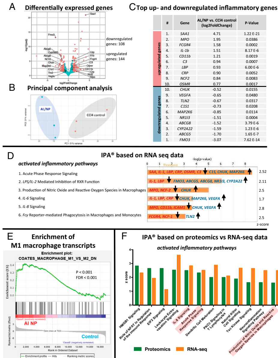
Fig. 5. Comparative transcriptomic and proteomic analyses by high-throughput RNA-seq (supported by mass spectrometry proteomics) of representative liver samples from AL/NP-treated (4 mg/kg AL) vs. untreated CCl 4 fibrotic livers (each n = 3). (A) Volcano plot and numbers of significantly differentially expressed genes between AL/NP-treated and fibrotic mice. Differentially expressed genes with log 2 -fold change ≥ 1 or ≤ -1 and FDR ≤ 0.05 are shown in red, and the top 10 up- and down-regulated inflammatory genes are labeled. (B) Principal component (PC) analysis based on RNA-seq data indicates clustering of AL/NP-treated vs. CCl 4 control mice (PC1 51% and PC2 21% variance, respectively). (C) Top 10 up- and down-regulated genes associated with inflammation as determined by RNA-seq ( padj , P values adjusted for multiple testing by the Benjamini-Hochberg method). (D) Relevant immune-related signaling pathways, which were found to be activated as predicted by IPA based on RNA-seq differential expression data (bars represent P values adjusted for multiple testing by the Benjamini-Hochberg method, the yellow line indicates the ratio of molecules which are regulated in a given pathway and meet the cutoff criteria, and the involved up- and down-regulated genes are mentioned). (E) GSEA of differentially expressed genes in AL/NP-treated livers, compared with CCl 4 fibrotic control livers, identified highly enriched genes in gene sets related to M1- vs. M2-type macrophages ( P < 0.001, FDR < 0.001). (F) Comparative IPAs of activated inflammatory pathways for RNA-seq vs. proteomics data obtained from quantitative proteomic analysis by mass spectrometry (the three most significant pathways identified by RNA-seq IPAs are highlighted in red). Proteomic analysis supported the previous transcriptomic results, corroborating that macrophage-repolarizing inflammatory pathways are activated by AL/NP treatment.
