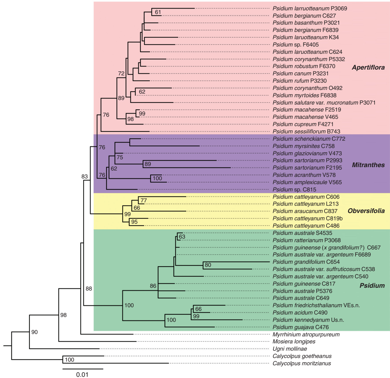
FIG. 2. Maximum likelihood phylogenetic tree of Psidium L. with 31 species (45 accessions). Numbers to the right of nodes are bootstrap values. Section names are to the right of clades. Vouchers are identified by the first letter of the first collector’s surname and number. For complete voucher data, see Supplementary data Tables S1 and S3 .
