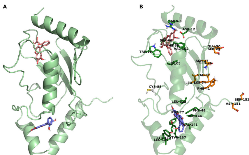
Figure 10. Computational docking of NSC 9037 to Rad6B
