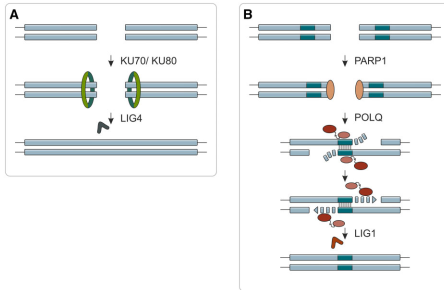
Figure 1 DSB repair via NHEJ. A DSB can be repaired via cNHEJ (A) or aNHEJ (B). In cNHEJ-mediated repair, the broken ends are bound by the KU70/KU80 heterodimer (green) and re-ligated by LIG4 (gray). Depending on whether the ends need to be processed prior to re-ligation, small insertions and/or deletions may occur in addition to error-free repair. In contrast, microhomologies (dark blue) at the break site are used in aNHEJ-mediated repair. Here, the break ends are bound by the polymerase PARP1 (orange), initiating the 5'- to 3'-resection of the ends. The annealing of the exposed microhomologies takes place, stabilized by the polymerase POLQ (red), whereby intervening regions can get lost. After filling the gaps via a POLQ-mediated fill-in synthesis, the break can be ligated. As areas between the microhomologies are resected, aNHEJ-mediated repair results in large deletions or more complex insertions.
