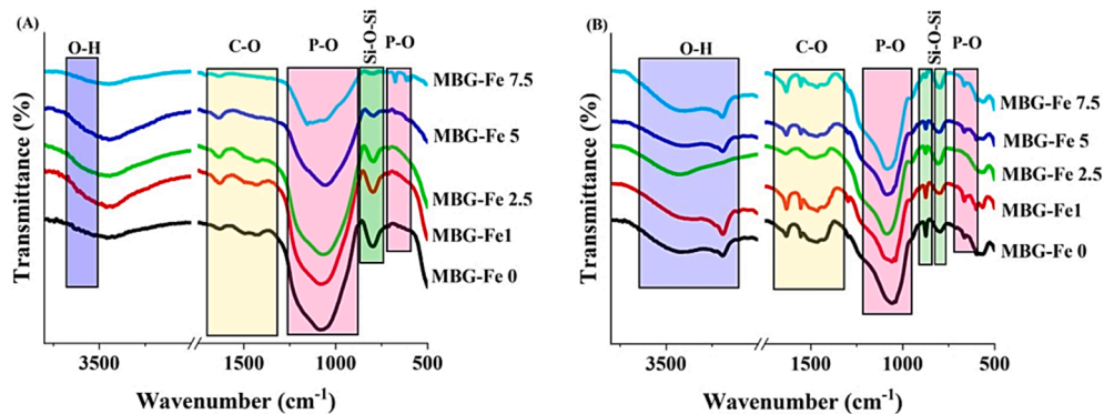
Fig. 4. FTIR spectra of the undoped and Fe 2 O 3 -doped MBGs before (A) and after 7 days of incubation in SBF (B).
