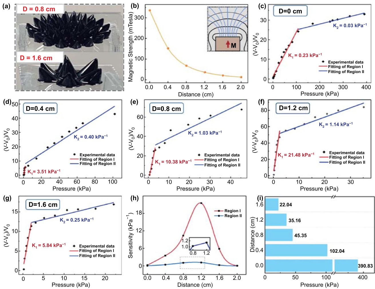
Fig. 3 Pressure sensing performance under different distances ( D ) with magnet. a Photograph of diverse formations of ferrofluid at different distances. b Characterization of the magnetic field strength generated under different distances. The inset shows the magnetic induction line in the direction of distance change. c-g The summarized relationship and linear fitting between the relative variations of voltage and the pressure applied on the device under different distances with magnet, from 0 to 16 mm at 4 mm intervals. The summarized variation of h sensitivity and i detection range of pressure sensor under different distances with magnet
