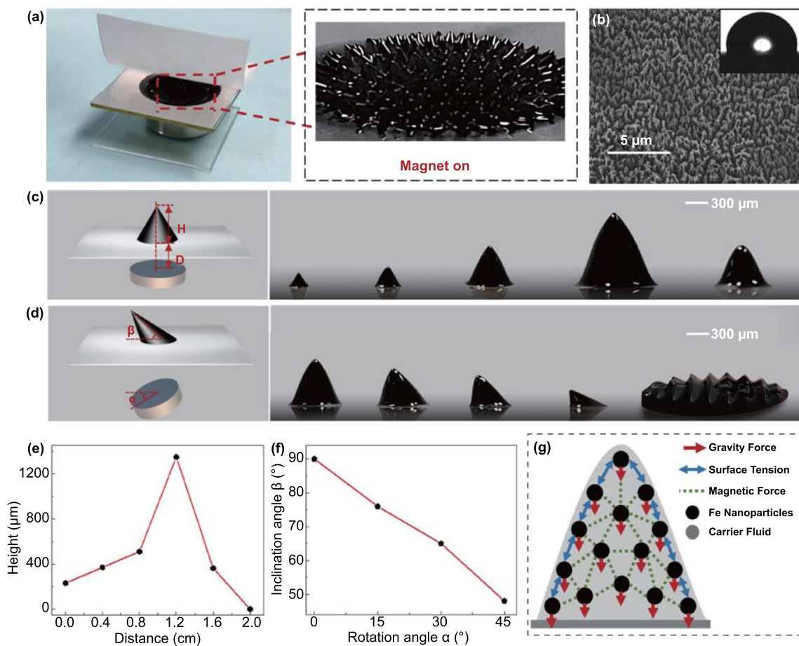
Fig. 1 Dynamic behaviors of the ferrofluid. a Photograph of FTTS. Inset displays the topography of microstructure in response to magnetic field. b The SEM image of PTFE membrane used to contact with ferrofluid, scale bar 5 \mu\text{m} . Inset shows the photograph of its contact angle. Schematic illustration and real-time microscope images of the dynamic behaviors of the ferrofluid in response to changing c distance and d angle with the magnet, scale bar 300 \mu\text{m} . Quantitative relations between different magnet conditions and geometric parameters of ferrofluid spikes: e distance and height, f rotation angle and inclination angle. g Force analysis of ferrofluid under magnetic field
