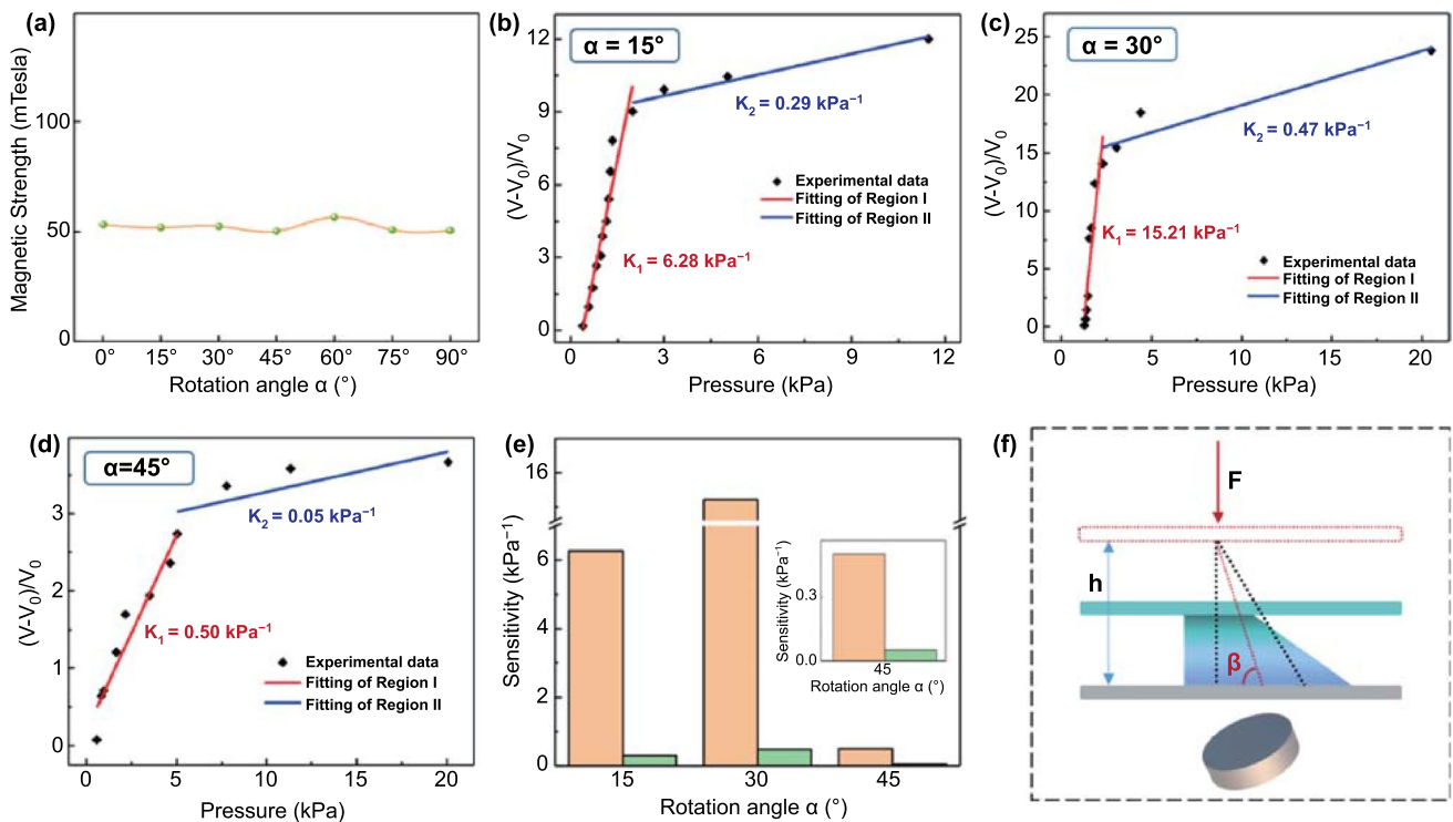
Fig. 4 Pressure sensing performance under different angles ( \alpha ) with magnet. a Characterization of the magnetic field strength generated under different angles. b-d The summarized relationship and linear fitting between the relative variations of voltage and the pressure applied on the device under different angles with magnet, from 15^\circ to 45^\circ at 15^\circ intervals. e The summarized variation of sensitivity of pressure sensor under different distances with magnet. f Force analysis diagram when tilted ferrofluid spike is pressed
