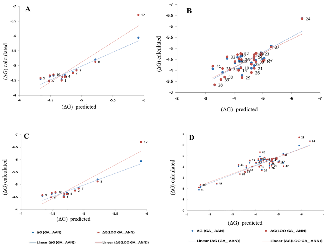
Fig. 6. The diagram of ( \Delta G ) values from docking versus the predicted ( \Delta G ) values from the GA-SW-MLR models for phosphosphonat compounds. A) model 1, B) model 2, C) model 3, and D) model 4.
