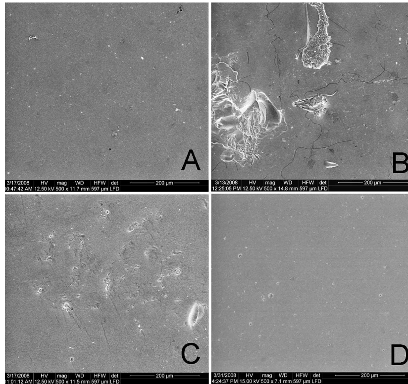
Figure 5. SEM images from the PA + S group. (A) Autoglaazed (baseline). (B) After resin removal. (C) After porcelain polishing kit. (D) After diamond polishing paste.
