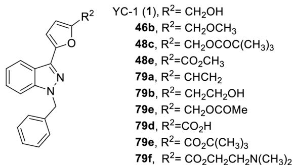
Fig. 21 Structure of YC-1 analogs (48, and 79).
