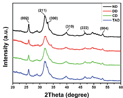
Fig. 7 XRD patterns of the dentin surface of natural dentin (black line), demineralized dentin (red line), C-dentin (green line), and the TA-dentin (blue line).
