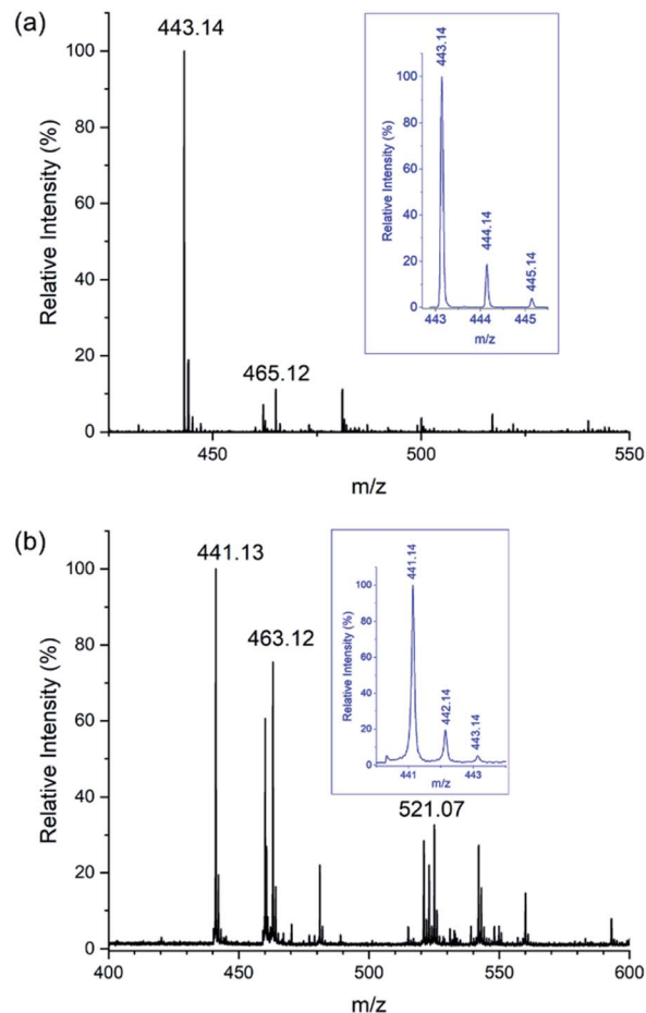
Fig. 9 ESI mass spectra recorded in negative mode of samples containing acetonitrile: water (9 : 1). Samples were diluted from aqueous solutions containing \text{Na}[\text{Sb}(\text{DOTA})] \cdot 4\text{H}_2\text{O} (0.5 mM) incubated with \text{Ca}(\text{NO}_3)_2 \cdot 4\text{H}_2\text{O} (1 mM) at 298 K showing the replacement of \text{Sb}^{3+} with \text{Ca}^{2+} recorded in: (a) positive mode with peaks corresponding to [\text{H}_3\text{Ca}(\text{DOTA})]^+ ( m/z 443.14) (expanded in inset) and [\text{NaH}_2\text{Ca}(\text{DOTA})]^+ ( m/z 465.12) and (b) negative mode with peaks corresponding to [\text{HCa}(\text{DOTA})]^- ( m/z 441.14) (expanded in inset), [\text{NaCa}(\text{DOTA})]^- ( m/z 463.12), and [\text{Sb}(\text{DOTA})]^- ( m/z 521.07).
