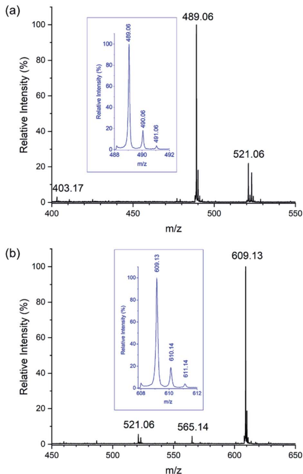
Fig. 8 ESI mass spectra recorded in negative mode of samples containing acetonitrile : water (9 : 1). Samples were diluted from aqueous solutions containing \text{Na}[\text{Sb}(\text{DOTA})] \cdot 4\text{H}_2\text{O} (0.5 mM) incubated at 298 K with (a) \text{Y}(\text{NO}_3)_3 \cdot 6\text{H}_2\text{O} (0.5 mM) showing almost complete replacement of the \text{Sb}^{3+} with \text{Y}^{3+} showing peaks corresponding to [\text{Y}(\text{DOTA})]^- ( m/z 489.06), [\text{Sb}(\text{DOTA})]^- ( m/z 521.06), and [\text{H}_3\text{DOTA}]^- ( m/z 403.17), and with (b) \text{Bi}(\text{NO}_3)_3 \cdot 5\text{H}_2\text{O} (0.5 mM), showing almost complete replacement of \text{Sb}^{3+} with \text{Bi}^{3+} with peaks corresponding to [\text{Bi}(\text{DOTA})]^- ( m/z 609.13), [\text{Bi}(\text{DOTA})-\text{CO}_2]^- ( m/z 565.14), and [\text{Sb}(\text{DOTA})]^- ( m/z 521.06).
