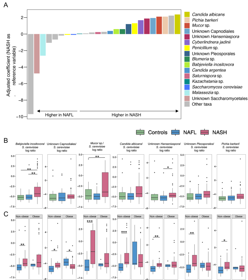
Figure 2. Compositional changes in the fecal mycobiome of patients with NASH. (A) Differential abundance of fungal taxa among groups were calculated using Songbird under consideration of clinical metadata (age, gender, BMI, type 2 diabetes, proton pump inhibitor use and alcohol consumption). Fungal taxa with at least 90% confidence level alignment in the UNITE database were colored. (B) Log-ratios of specific fungal taxa that were significantly different among groups, either when including all patients, or (B) when investigating subgroups based on obesity. We determined the denominator for the calculation of the log-ratios by choosing a fungal taxon that is present in all samples. This was the case for Saccharomyces cerevisiae ( S. cerevisiae ). In order to handle problems occurring when calculating log-ratios in zero-inflated microbiome data, we added a constant small value (0.1) to each count before calculating log-ratios. In (A-C), 78 patients with NAFLD were included in the analysis of whom 24 had NAFL, 54 had NASH. Of the patients with NAFL, 17 (70.8%) were non-obese and 7 (29.2%) were obese. Of the patients with NASH, 21 (38.8%) were non-obese and 33 (61.2%) were obese. In (B-C), 16 subjects without any known disease were additionally included. P values determined by Kruskal-Wallis test with Dunn’s post-hoc test for skewed distributions followed by false discovery rate (FDR) or Whitney-Wilcoxon rank-sum test. * P <0.05, >0.01; ** P <0.01, P >0.001; *** P <0.001. For the box and whisker plots (b-c), the box extends from the 25th to 75th percentile, with the center line indicating the median; the bottom whiskers indicate the minimum values
