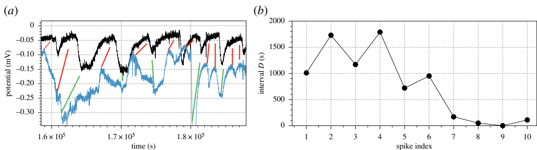
Figure 7. Exemplar synchronization of spikes in two neighbouring sporocarps of S. commune : channel (3–4), second sporocarp in figure 1b and channel (5–6), third sporocarp in figure 1b. (a) Spiking activity, corresponding spikes of increased voltage are linked by red lines and decreased voltage by green line. (b) Dynamics of the interval between spikes.
