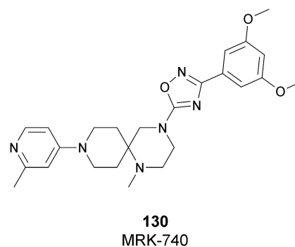
Fig. 36 PRDM9 inhibitor.
