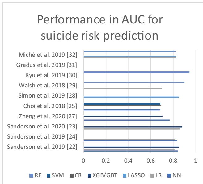
Figure 6. Performance in AUC of the different algorithms, based on the studies included in Table 1.
