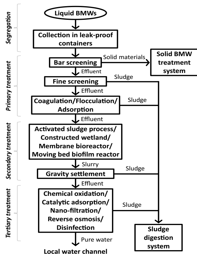
Fig. 4. Liquid BMW treatment procedure (Kaushal et al., 2022).
