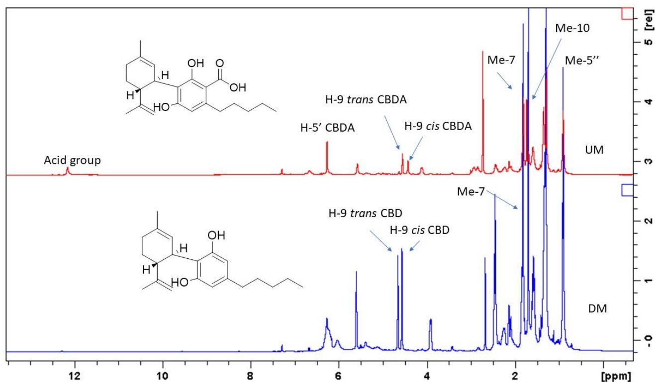
Figure 3. 1 H-NMR spectra showing the cannabinoid profiles of UM and DM chloroform extract.
