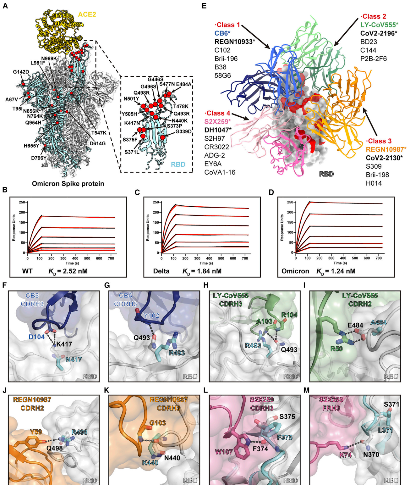
Figure 2. Analysis of the Omicron spike RBD mutations in ACE2 binding and antibody evasion
