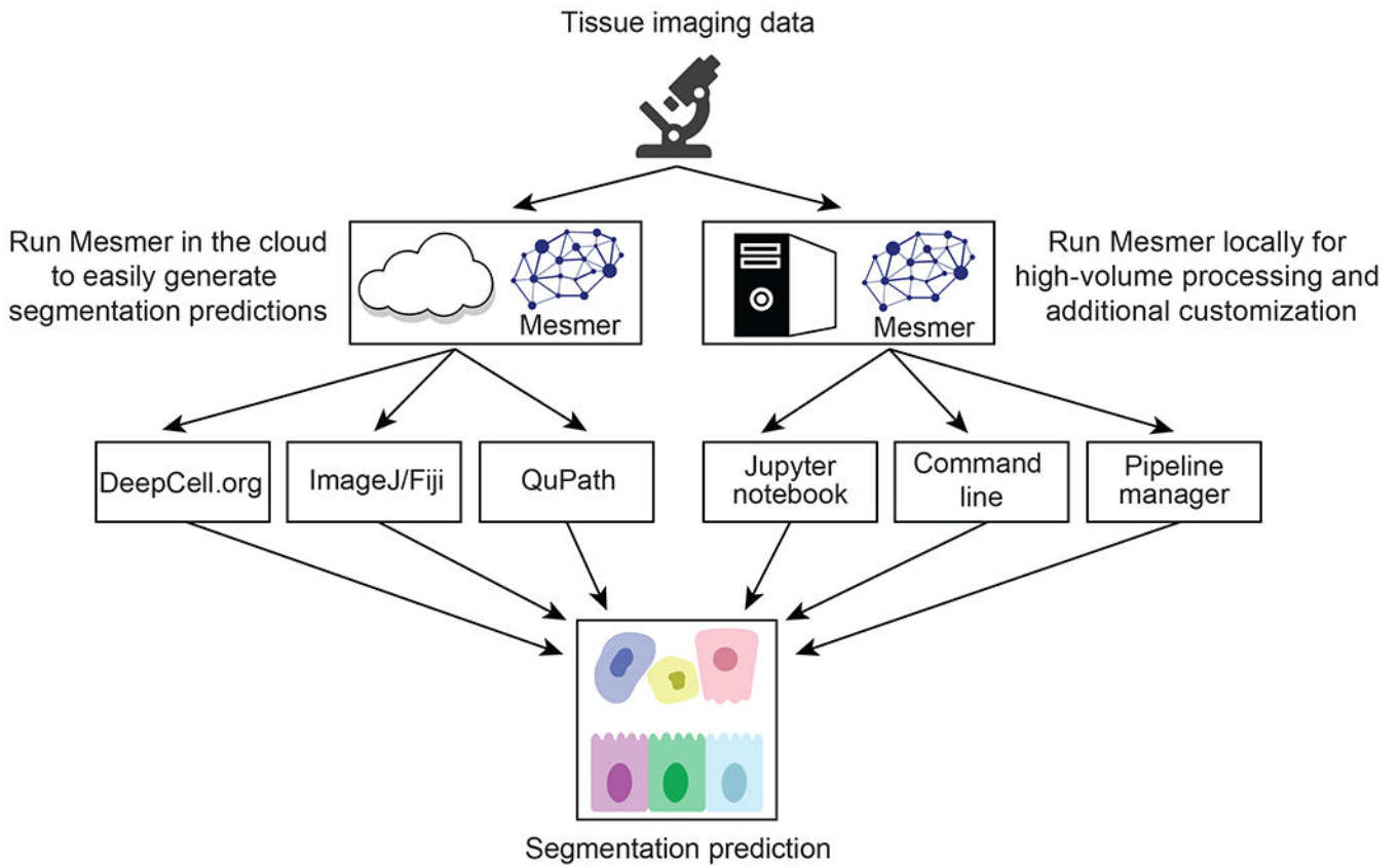
Figure 6: Cloud-native and on-premise software facilitates deployment of Mesmer.
