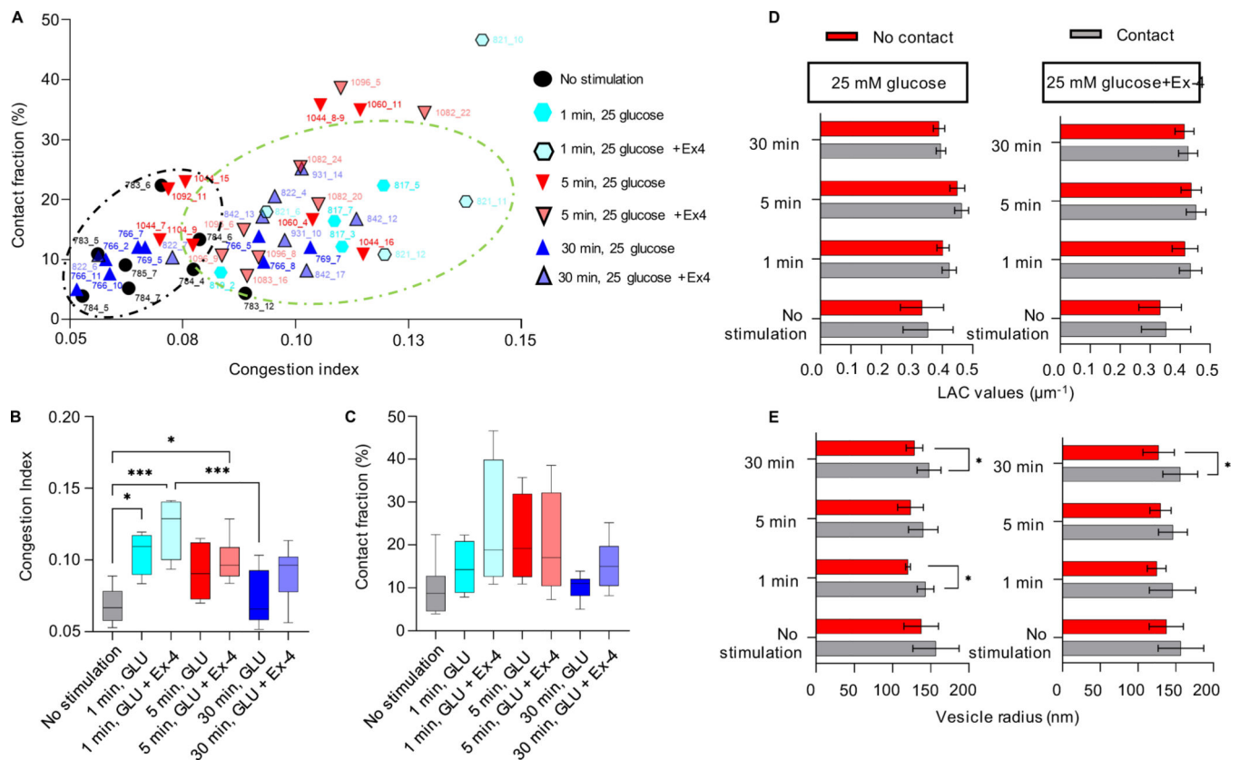
Figure 5: Analysis of the mitochondria-insulin vesicle interaction randomness.
