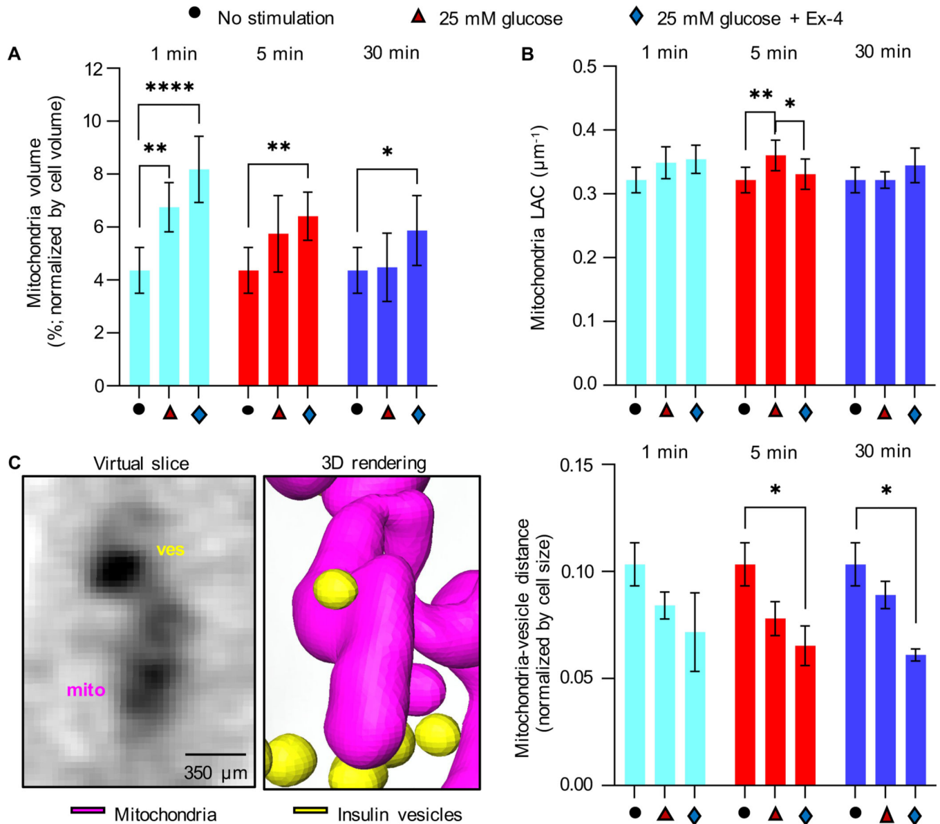
Figure 2: Effect of glucose and Ex-4 stimulation on mitochondria properties and spatial distribution.
