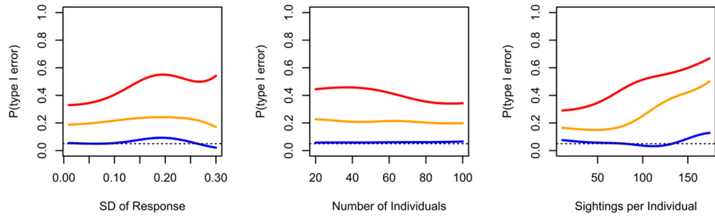
Figure 2. Conditional probability plots from dyadic regression simulation. Lines indicate smoothed conditional probabilities of a type I error (a p -value less than 0.05) for datastream permutations using the coefficient (red) or t -value (orange), and node-label permutations (blue) in relation to three covariates. Dotted line indicates target type I error rate of 0.05.
