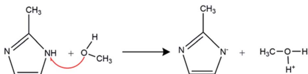
Scheme 2 Reaction scheme of Hmim deprotonation in methanol.
