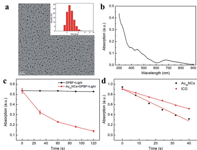
Fig. 2 (a) TEM image and size distribution of \text{Au}_{25}\text{NCs} . (b) UV-Vis absorption spectra of \text{Au}_{25}\text{NCs} . (c) Singlet oxygen generation of \text{Au}_{25}\text{NCs} . Time dependent absorption changes at 412 nm of DMF solutions of DPBF (200 \mu\text{M} ) and \text{Au}_{25}\text{NCs} (0 or 200 \mu\text{g mL}^{-1} ) mixture upon irradiation at 808 nm light. (d) Singlet oxygen generation efficiency liner fitting of \text{Au}_{25}\text{NCs} and indocyanine green (ICG).
