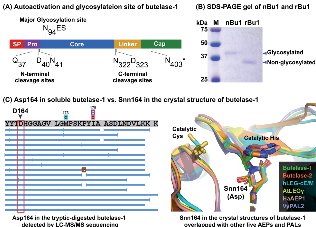
Fig. 3 Proteomic characterization of nBu1 and activated rBu1. (A) Determination of auto-activation sites and N -glycosylation site. N403* estimated cleavage site based on intermediate band size and LC-MS/MS sequencing data. (B) Coomassie blue-stained SDS-PAGE gel of nBu1 and the activated rBu1. nBu1, calculated molecular weight (MW) = 32 kDa, observed MW \approx 38 kDa. rBu1, calculated MW = 31 kDa, observed MW \approx 37 kDa. (C) Detection of Asp164 in the soluble butelase-1 by LC-MS/MS sequencing in contrast to the Snn164 in the crystal structure of rBu1 superimposed with other AEPs and PALs. Left panel shows one example of MS/MS sequencing of tryptic digested butelase-1 fragments (image obtained by PEAK Studio after DB search and PTM analysis). Right panel includes structures with PDB codes: butelase-1 (6DHI), butelase-2 (6L4V), human legumain–cystatin E/M complex (4N6O), AtLEG \gamma (5OBT), HaAEP1 (6AZT), and VyPAL2 (6IDV).
