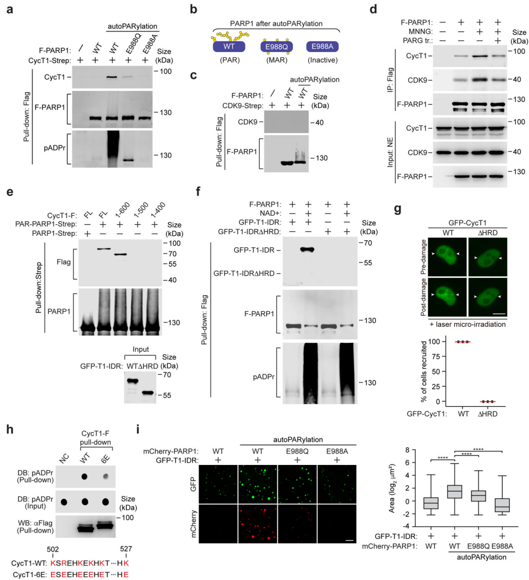
Figure 2. The PARP1-CycT1 binding depends on the histidine-rich domain of CycT1 and the PAR chains on PARP1 and is likely facilitated by electrostatic interactions between the two. a, c, e, & f, Purified and immobilized WT or mutant F-PARP1 or PARP1-Strep was subjected to autoPARylation reaction in vitro. The pattern of ADP-ribose attached on WT and mutant PARP1 after the reaction is diagrammed in b . After the reactions were stopped, the unmodified or modified PARP1 was incubated with purified CycT1-Strep ( a ), CDK9-Strep ( c ), full-length (FL) or truncated CycT1-F ( e ) or WT or the HRD-deleted GFP-CycT1-IDR ( f ). The input and pull-down proteins were analyzed by Western blotting (WB). d, HeLa cells expressing F-PARP1 or not were untreated or treated with MNNG. anti-Flag immunoprecipitates (IP) were incubated with recombinant PARG or not and then examined by WB. g, HeLa cells expressing WT or the HRD-deleted GFP-CycT1 were subjected to laser microirradiation and analyzed and quantified as in Fig.1i. Scale bar = 10 μM. The error bars indicate mean ± s.d. with n = 3 independent experiments. h, Purified and immobilized WT or mutant CycT1-F was incubated with autoPARylated PARP1. The
