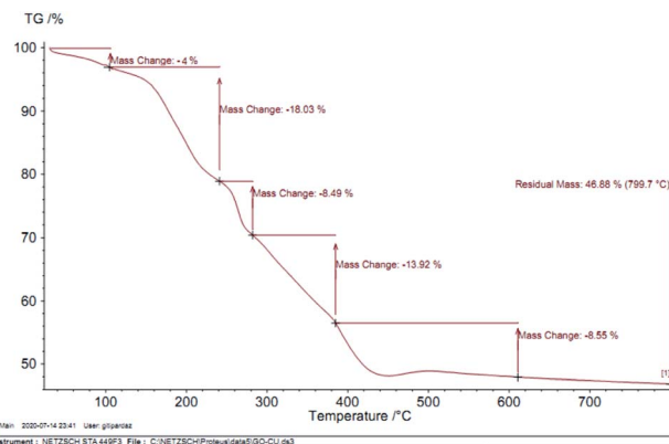
Fig. 6 TGA curve of Cu-ninhydrin@GO-Ni MNPs.
