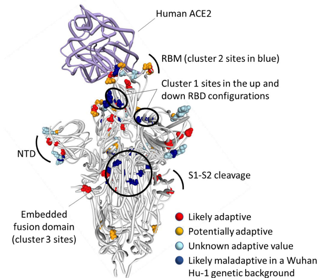
Fig. 3. Distribution of BA.1 amino acid replacements on the three-dimensional SARS-CoV-2 Spike trimer. In this rendering of the trimer, one protomer subunit is shown in the “up” or “open” configuration while interacting with human ACE2 (Xu et al. 2021). The other two subunits are in the “down” or “closed” configurations. Amino acids are color coded according to their likely contribution to viral adaptation in a Wuhan-Hu-1-like genetic background based on (1) patterns of synonymous and nonsynonymous substitutions at the codons encoding these amino acids in non-Omicron sequences, (2) patterns of mutational convergence between viruses in different VOCs, and (3) increases in the frequency over time of VOC sublineages encoding amino acids that match those found in BA.1. NTD, N-terminal domain, RBD, Receptor-binding domain; RBM, receptor-binding motif. Locations of sites in the three clusters of BA.1 mutations that are rarely seen and fall at either negatively selected (dark blue) and neutrally evolving (light blue) sites. An interactive version of this figure can be found here: https://observablehq.com/@stephenshank/sars-cov-2-ace2-protein-interaction-and-evolution-for-omicr .
