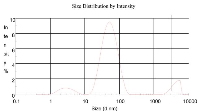
Fig. 4 Size distribution of the AuNPs synthesized from the Manilkara zapota leaf extract.
