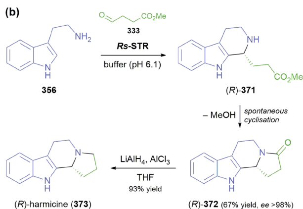
Scheme 47 ( R )-Selective Pictet–Spengler reactions of strictosidine synthases (STRs): (a) 1-alkyl-tetrahydro- \beta -carbolines obtained from tryptamine (356) and small, aliphatic aldehydes, (b) two-step chemo-enzymatic synthesis of ( R )-harmicine (373).
