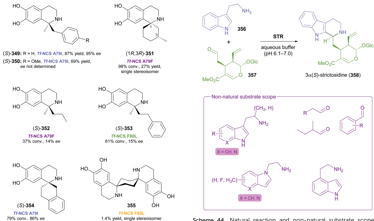
Fig. 5 Examples of 1,1-disubstituted and spirocyclic tetrahydroisquinolines obtained by NCS reactions of open-chain or cyclic ketones.
