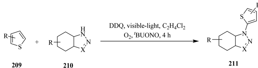
Scheme 73 DDQ-photocatalyzed direct C 2 -H amination of thiophene under visible-light irradiation.
