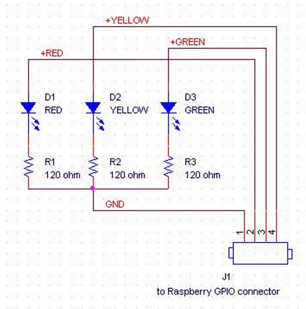
Fig. 13. The check light board schematic.
