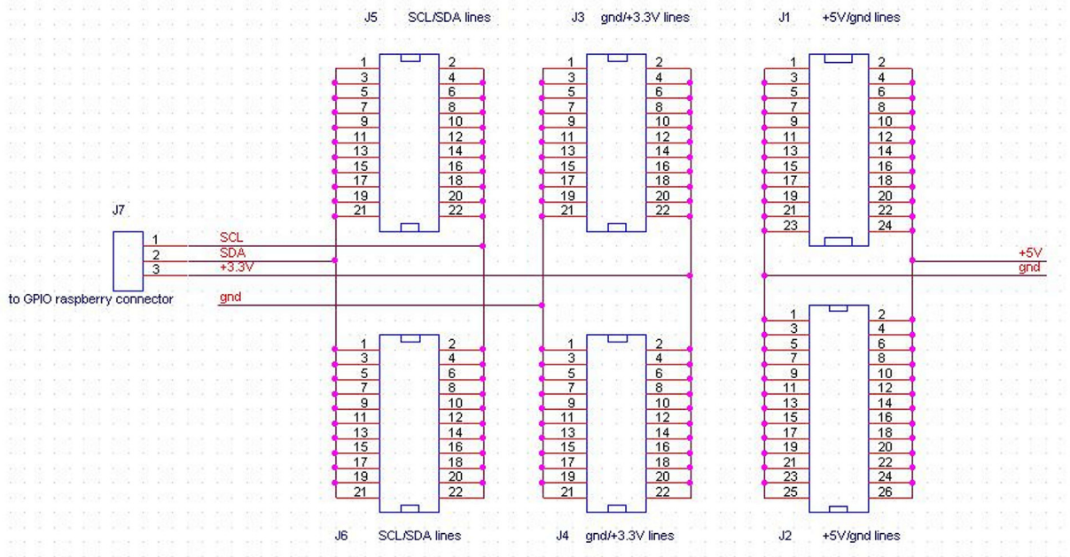
Fig. 11. The expansion board schematic.
