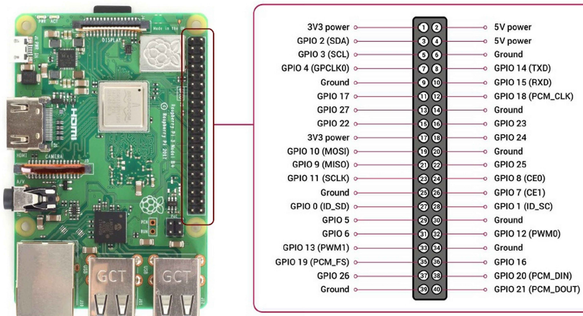
Fig. 4. The system mainboard, represented by a raspberry 3B+. Its GPIO connector is detailed on the right along with the pin function description.
