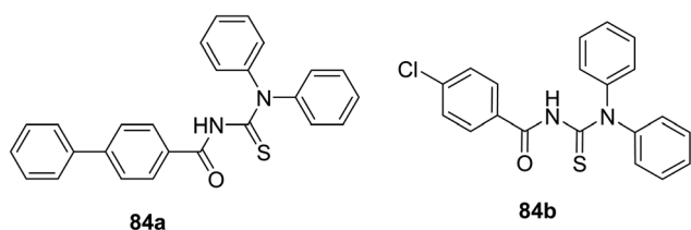
Scheme 27 Thiocarbamides 84a–b.
