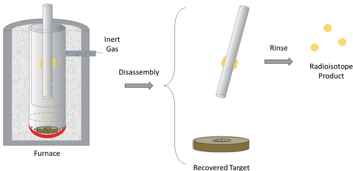
Fig. 4 Thermochromatographic dry distillation. Schematic depicting the separation of volatile PET radioisotopes from non-volatile target material after heating is performed in a furnace. The PET radioisotope condenses on a removable, cooler surface within the furnace. The radioisotope is removed from the surface using a rinse.
