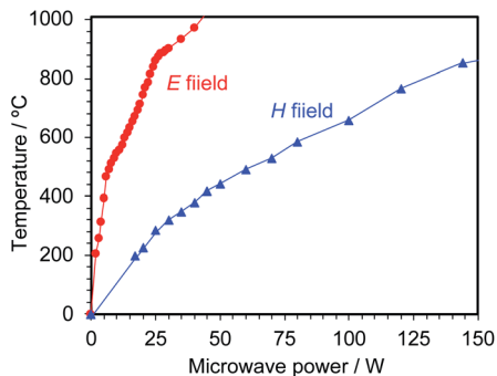
Fig. 3 Temperature change of the AC particulates in the 4 mm quartz reactor with respect to the microwave output power under E -field and H -field microwave heating conditions in the single-mode applicator.
