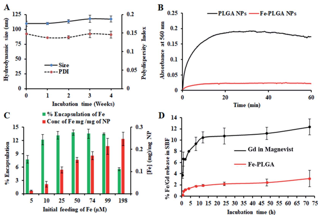
Fig. 2 Stability and loading/release study of iron(III) chelated polymeric NPs. (A) Stability of NPs over 4 weeks period when stored at 4 ^\circ\text{C} showing the change of size and polydispersity index. (B) serum stability test to measure dynamic aggregation of PLGA NPs and Fe-PLGA NPs using 90% fetal bovine serum environment to find the rapid increase in optical density of 560 nm due to NPs aggregation by forming protein corona, (C) iron loading efficiency with the different initial feeding concentration of \text{Fe}^{3+} per mg PLGA, and (D) a comparative Fe and Gd release study from Fe-PLGA NPs and Magnevist® in simulated body fluid (SBF), respectively. Data represents mean \pm S.D, n = 3 .
