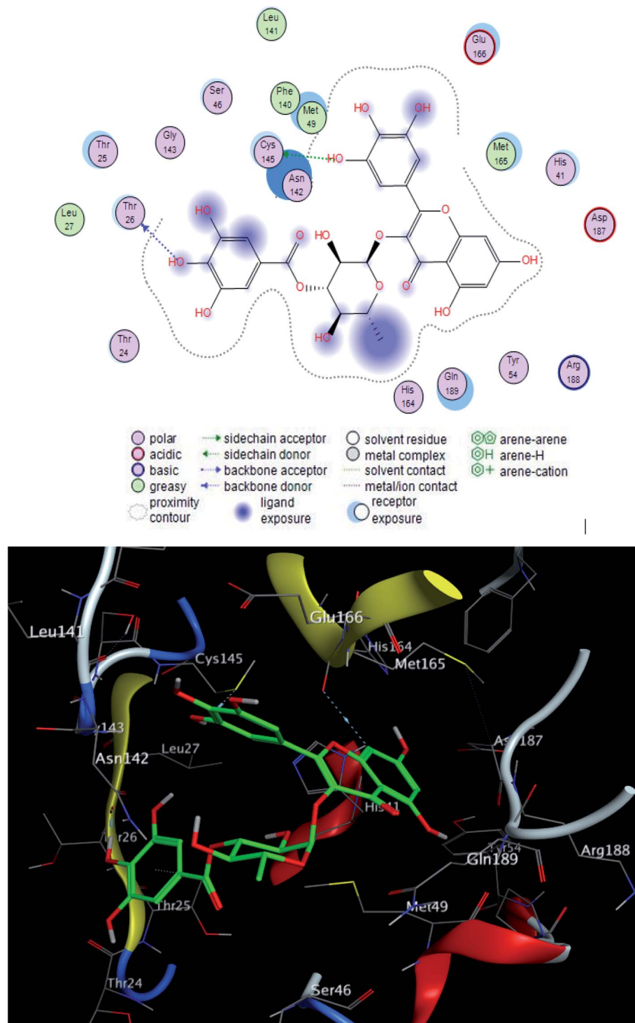
Fig. 4 2D and 3D ligand interactions of compound 3 with main protease receptor.
