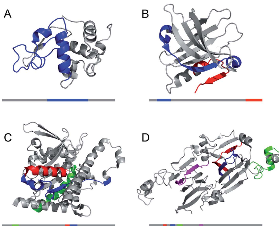
Fig. 8 The structural properties of PNF-forming peptides in the native structures of the proteins they originate from. The grey bars below the structures represent the protein sequences with the peptide positions indicated in the same colours. (A) Hen egg lysozyme (residues 53–100, 113 PDB ID 1JPO). (B) Bovine \beta -lactoglobulin (residues 12–32 and 138–162, 109 PDB ID 2Q2M). (C) Patatin from potato (residues 36–60, 224–240 and 247–266, 72 PDB ID 4PK9). (D) Soybean glycinin and \beta -conglycinin. The protein subunits have high structural similarity and peptides from different subunits are illustrated in the structure of \beta -conglycinin subunit \beta . 73
