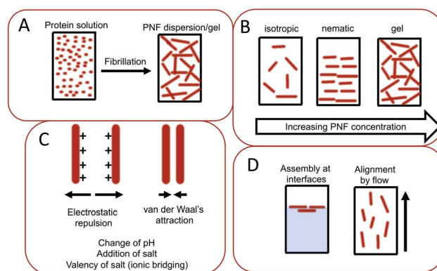
Fig. 13 Illustration of important parameters during assembly of PNFs into macroscopic materials. (A) The conversion of a protein into PNF results in changes of physical properties, such as increased viscosity and sometimes even gel-formation. (B) Depending on the PNF concentration different phases can form including non-ordered isotropic phases, liquid crystalline phases such as the nematic phases, or gels. (C) The PNF dispersion is stabilized by electrostatic repulsion, which counteracts close contacts between PNFs where van der Waals interactions will be strong. The electrostatic repulsion can be influenced by variations in parameters such as pH, salt concentration, and addition of multivalent ions that may enable ionic bridging. (D) PNFs are amphiphilic and tend to be enriched at interfaces. PNFs may also be aligned by applying flow.
