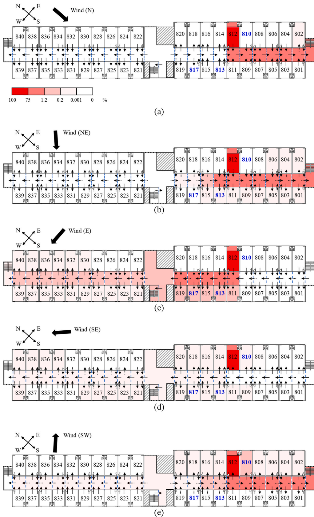
Fig. 6. Illustration of net airflow through the main internal openings and the normalised bio-aerosol concentrations (in %) at times characterised by different wind directions. Plots show the patterns of net airflow on the eighth floor of Luk Chuen House (under Scenario 1 [All doors closed].) with (a) a northerly wind at 11:00 on 24 May, (b) a north-easterly wind at 19:30 on 22 May, (c) an easterly wind at 15:00 on 23 May, (d) a south-easterly wind at 17:30 on 23 May, and (e) a south-westerly wind at 24:00 on 24 May in the year of 2020. The degree of transparency of the red square in each zone is inversely (but not proportionally) related to its normalised bio-aerosol concentration [refer to the colour scale in (a)]. The direction of net airflow is indicated by the black arrows, with a solid arrow indicating unidirectional airflow and a dashed arrow indicating bidirectional airflow.
