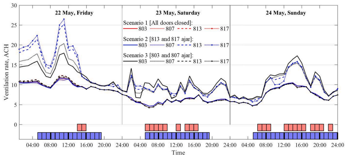
Fig. 9. Estimated hourly ventilation rates (ACH) for flats 803, 807, 813, and 817 in 3 scenarios, derived from the MIX program.
