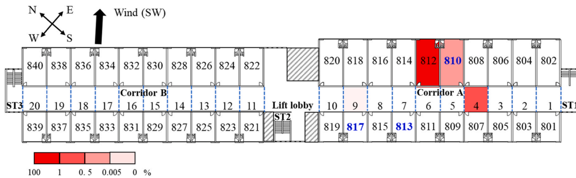
Fig. 7. Normalised tracer gas concentrations (%) in flats 810 and 812 and the corridors near the meshed window of flats 808 and 817 monitored at 17:47 on June 17, 2020.
