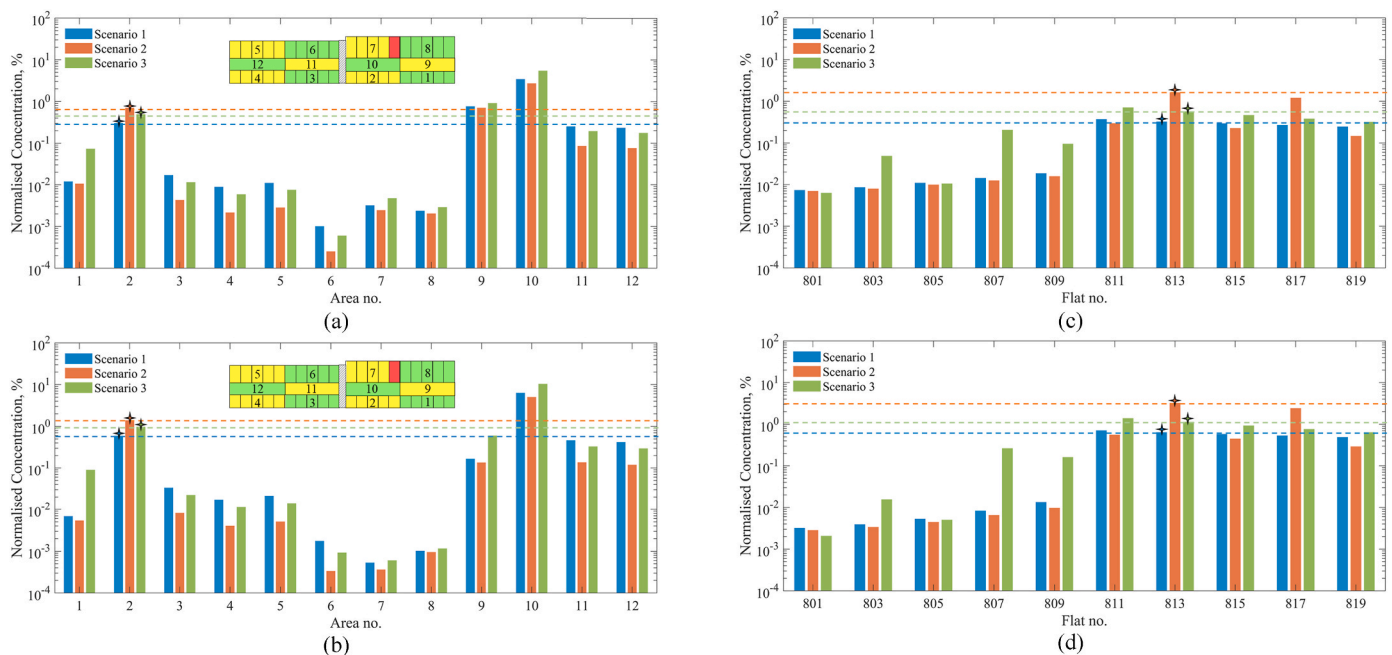
Fig. 8. Comparison of the average normalised bio-aerosol concentrations between the 12 areas, and between the flats in area 1 and area 2, under the three scenarios. (Scenario 1 [All doors closed], Scenario 2 [813 and 817 ajar] and Scenario 3 [803 and 807 ajar]). Plots show the average normalised bio-aerosol concentrations for (a) the 12 areas during index case’s home hours, (b) the 12 areas during suspected infection period for the secondary cases in flats 813 and 817, (c) the flats in area 1 and area 2 during the index case’s home hours, and (d) the flats in area 1 and area 2 during the suspected infection period for the secondary cases in flats 813 and 817. Note that values on the y-axis are presented on a log scale and the blue, brown, and green dashed lines notifies the corresponding normalised concentration in flats of area 2 ([a] and [b]) or flat 813 ([c] and [d]) in Scenario 1, 2, 3, respectively.
