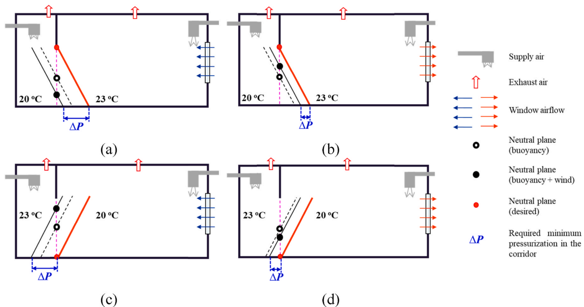
Fig. 11. Estimating the need for an imbalance in airflow or the over-supply of air to the corridor to avoid the escape of air from a guest room to the corridor. The \Delta P as shown in all plots is the minimum required pressurization in the corridor. The goal of design is to push the neutral plane at the doorway up or down such that no air is leaked from the room to the corridor (desired pressure profile: indicated by the solid red line). The neutral plane is located at mid-height when only a buoyancy force from differences in air density exists (buoyancy-driven pressure profile: indicated by the dotted line). When wind pressure also acts on the window, the neutral plane moves (wind- and buoyancy-driven pressure profile: indicated by the solid black line). Individual plots illustrate the movement of the neutral plane when (a) the guest room is warmer than the corridor, and a positive wind acts on the window, (b) the guest room is warmer than the corridor, and a negative wind acts on the window, (c) the guest room is cooler than the corridor, and a positive wind acts on the window, and (d) the guest room is cooler than the corridor, and a negative wind acts on the window.
