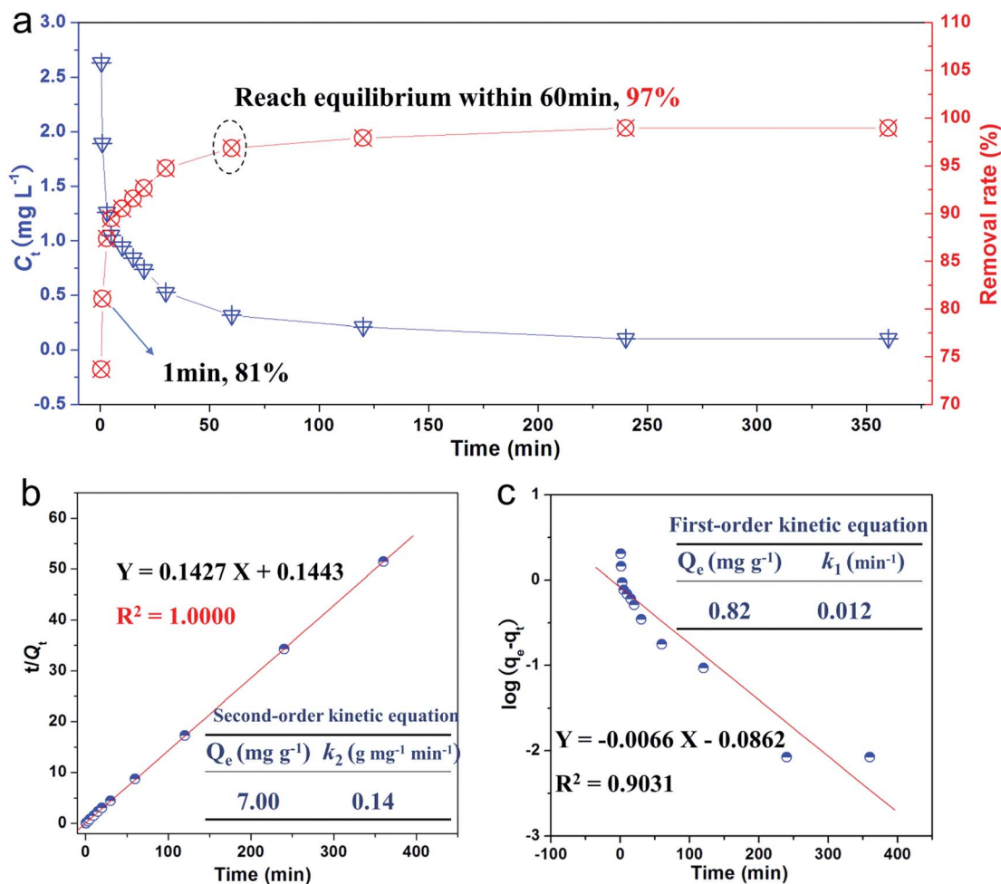
Fig. 3 (a) Adsorption kinetics of phosphate on L-NH 2 @Ce, and fitting results for (b) pseudo-second-order model and (c) pseudo-first-order model on L-NH 2 @Ce.
