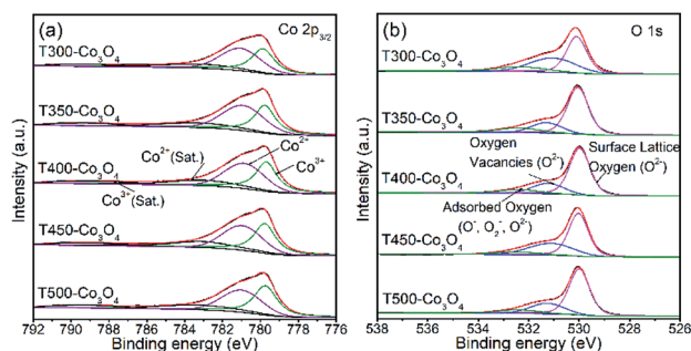
Fig. 8 (a) Co 2 p_{3/2} , and (b) O 1s XPS spectra of Co_3O_4 samples.
