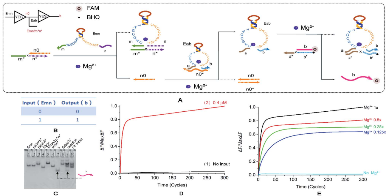
Fig. 3 (A) Reaction schematic diagram of the YES–YES cascade logic circuit. The fluorophore FAM is modified at the 5' end of the strand a^*b^* , the quenching BHQ is modified at the 3' end of the strand b , and the input DNAzyme Emn binds to the double strand n0/m^*n^* to replace the strand n0 . The strand n0 unlocks the DNAzyme Eab, which in turn reacts with the double strand b/a^*b^* to release the fluorescent strand b . (B) YES–YES logic circuit corresponding to the logical operation truth table. (C) Native PAGE analysis of the YES–YES logic circuit. The number is marked above each lane, and the top is the DNA strand type for each lane. Lane 1: DNAzyme Emn; lane 2: double stranded n0/m^*n^* ; lane 3: double strand formed by annealing of DNAzyme Eab to strand n0^* ; lane 4: double stranded b/a^*b^* ; lane 5: double strand formed by annealing of DNAzyme Emn with strand m^*n^* ; lane 6: double stranded n0/n0^* ; lane 7: strand b , which is the comparison strand of the result; lane 8: double strand formed by annealing of DNAzyme Eab and strand a^*b^* ; lane 9: reaction of YES–YES cascade logic circuit, input 1; and lane 10: YES–YES cascade input logic, no input reaction. Enter 0. The concentration ratio between the strands is 1 : 1. (D) The normalized fluorescence intensity curve of the YES–YES logic circuit, the solution concentration is 0.4 \mu\text{M} , and the sampling scan interval is set to 13 s for a total of 300 cycles. (E) YES–YES logic curve normalized fluorescence intensity as a function of \text{Mg}^{2+} concentration.
