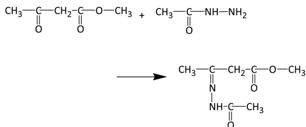
Fig. 8 Reaction of methyl acetoacetate and acetoaldehyde.
