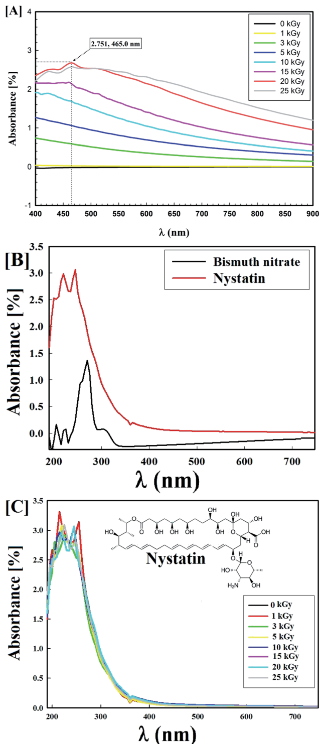
Fig. 1 UV-Vis spectra of the synthesized Bi 2 O 3 NPs-Nystatin, where [A] the initial screening results to obtain the most potent gamma-ray dose to be used for Bi 2 O 3 NPs-Nystatin synthesis, [B] UV-Vis spectra of the starting materials included in the Bi 2 O 3 NPs-Nystatin synthesis, and [C] stability of the nystatin drug after exposure to different gamma-ray doses.
