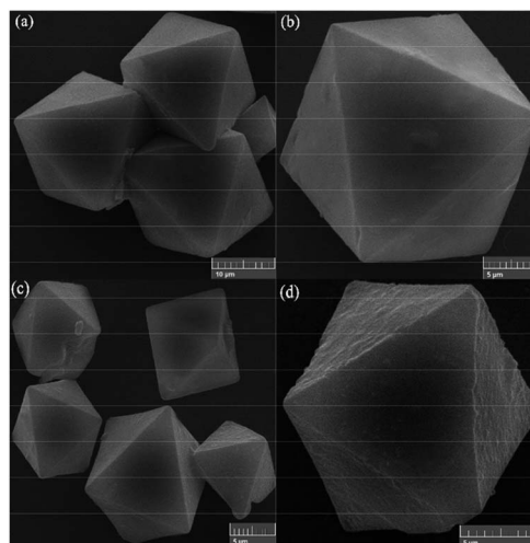
Fig. 2 SEM images of (a and b) HKUST and (c and d) HKUST-AMP-SO 3 H.
