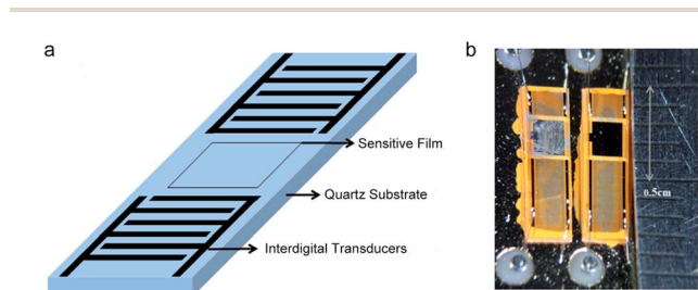
Fig. 1 (a) A schematic illustration, and (b) an optical microscope image of the ST-cut quartz SAW device.
