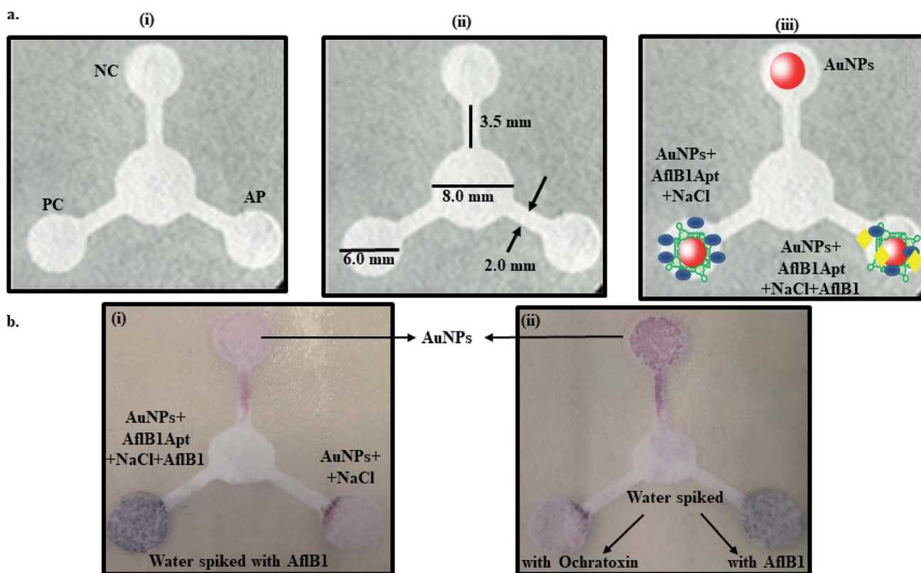
Fig. 4 Schematic representation of \mu PAD paper microfluidic device. (a) (i) Concept of \mu PAD—positive control (PC), negative control (NC), analyte pad (AP), (ii) dimensions and (iii) fabrication of the paper device; (b) (i) the color development after spiking Afl B1 in water and (ii) color development in presence of AflB1/no change in color in presence of ochratoxin in water.
